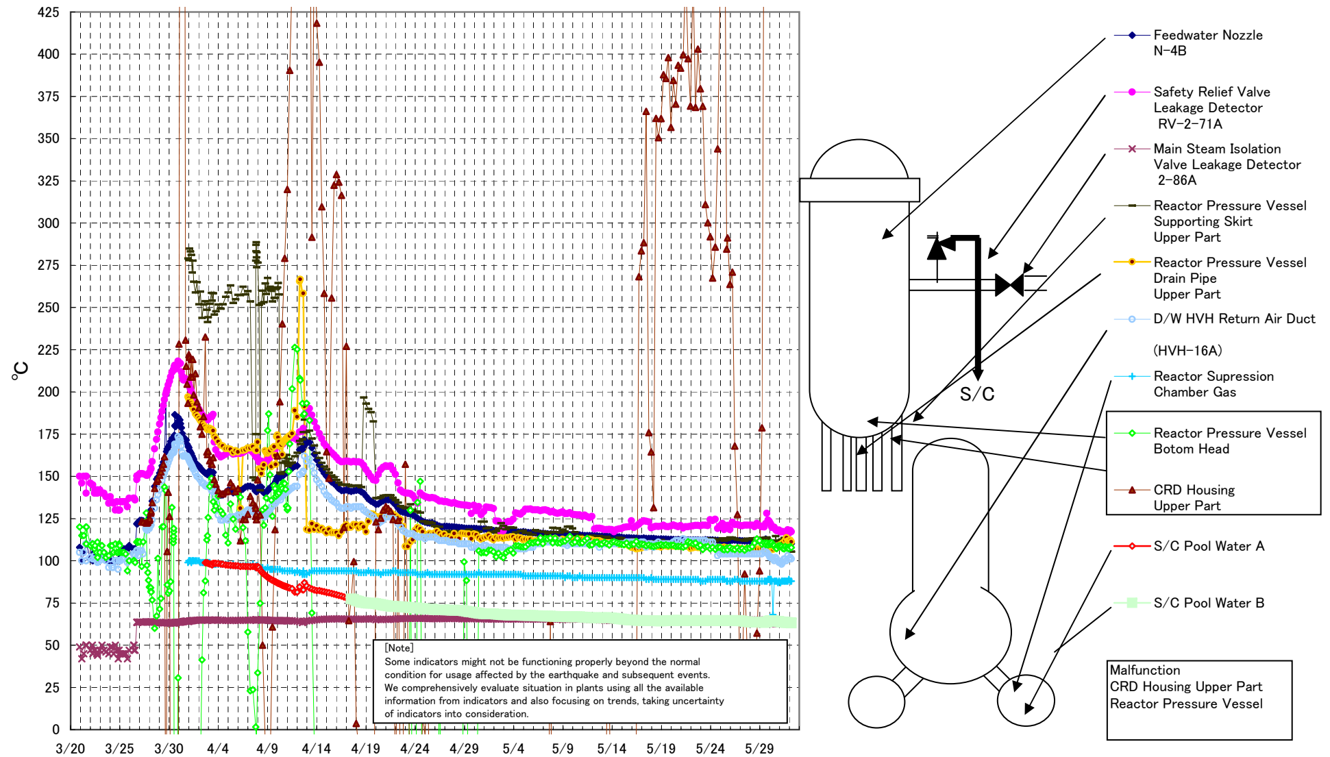
Fukushima Daiichi Nuclear Power Station Unit2 Parameters of Temperature (Typical Points)
